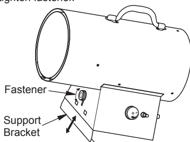
Figure 6 - Adjusting Heater Height Model PCFA60V
