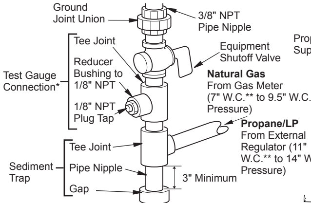
Figure 16 - Gas Connection
