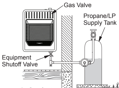
Figure 19 - Checking Gas Joints for Propane/LP Gas
