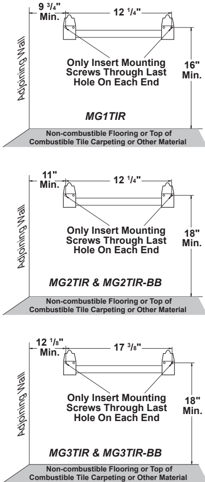
Figure 7 - Mounting Bracket Clearances
