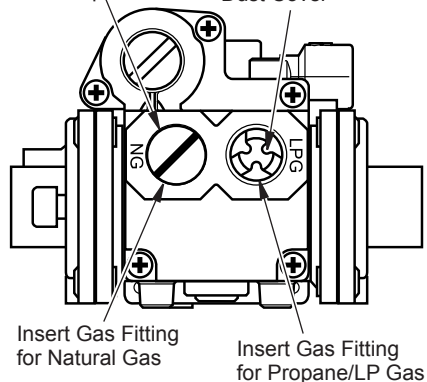
Figure 15 - Gas Regulator
