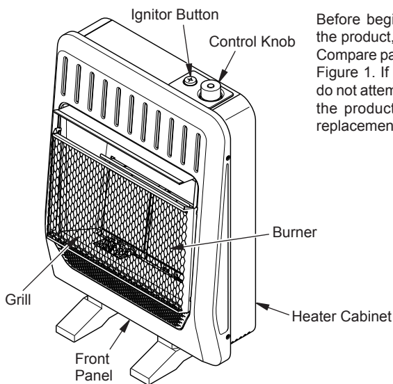
Figure 1 - Vent-Free Gas Heater MG2TIR Shown with Optional Base Feet
