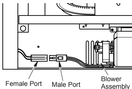
Figure 14 - Attaching Blower to Power Cord
