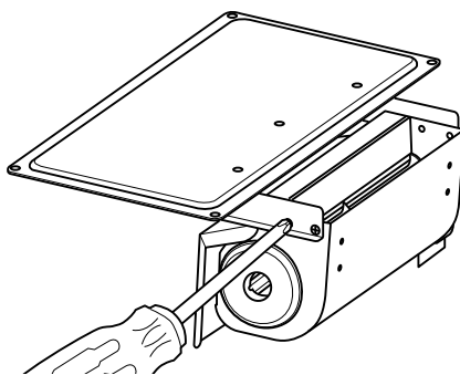
Figure 11 - Attaching Blower Assembly to Blower Access Panel
