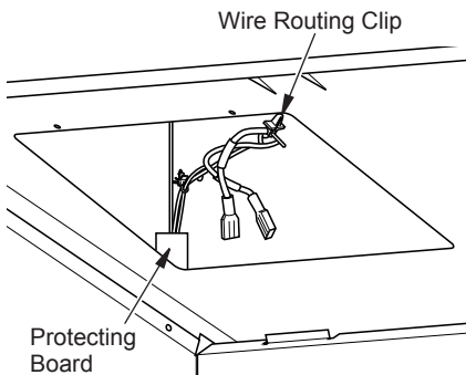
Figure 4 - Attaching Wiring
