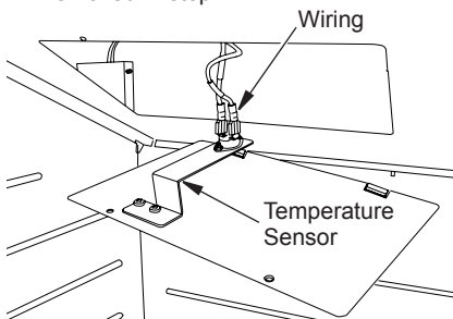
Figure 5 - Connecting Wires to Temperature Sensor
