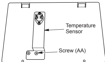
Figure 3 - Attach Temperature Sensor to Heat Insulation Board
