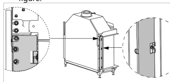
Figure 9: Removing the strip
