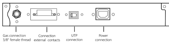
Figure 11b: E-box connections Gi80/140 series
