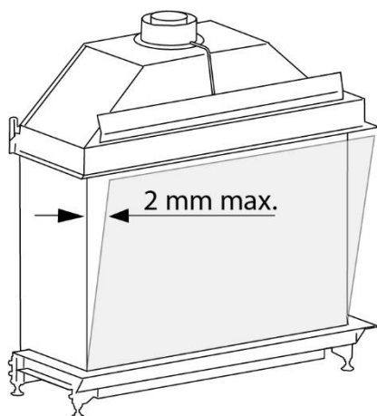
Figure 7: Check alignment front glass
