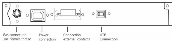
Figure 11a: E-box connections Gi75/59 series, Gi105/59 series, Gi105/79 series
