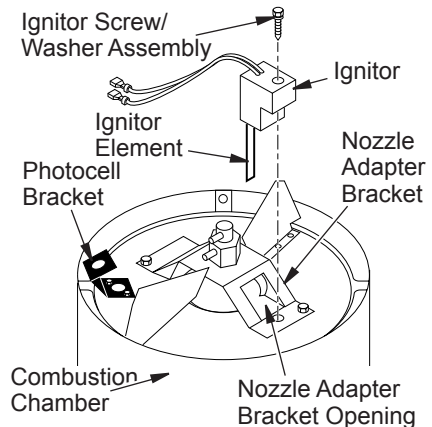
Figure 15 - Ignitor SP002-01 Replacement
