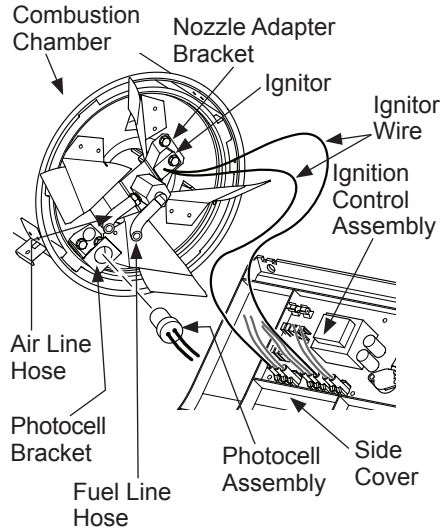
Figure 14 - Disconnecting Ignitor Wires from Ignition Control Assembly
