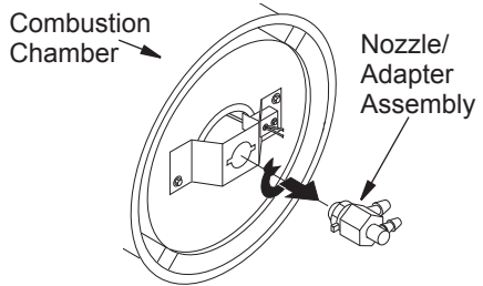
Figure 17 - Removing Nozzle/Adapter Assembly
