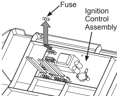
Figure 19 - Replacing Fuse
