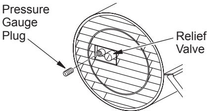
Figure 11 - Pressure Gauge Plug Removal
