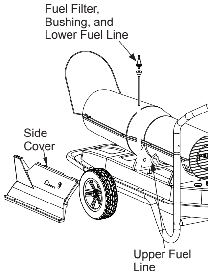
Figure 13 - Fuel Filter Removal
