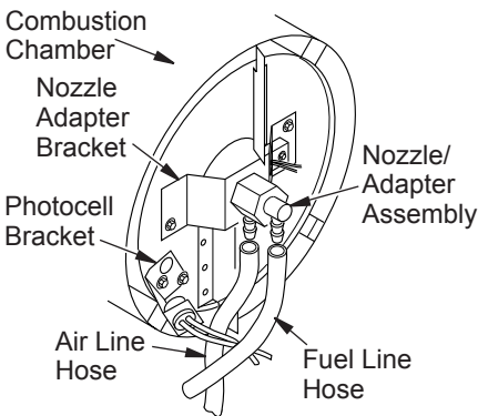
Figure 16 - Removing Air and Fuel Line Hoses
