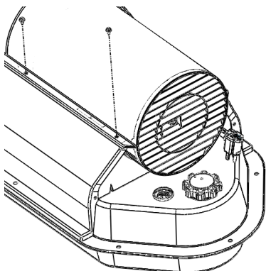
Figure 7 - Upper Shell Removal,
