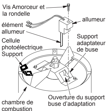
Figure 15 - Amorçeur SP002-01 Remplacement
