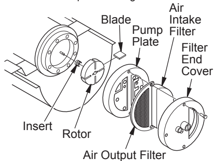
Figure 20 - Rotor Location
