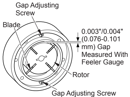
Figure 21 - Gap Adjusting Screw Locations
