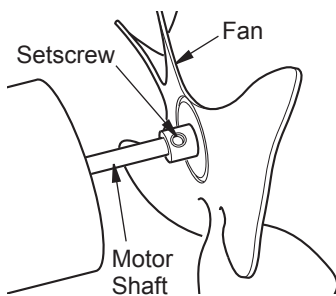
Figure 8 - Fan, Motor Shaft, and Setscrew Location
