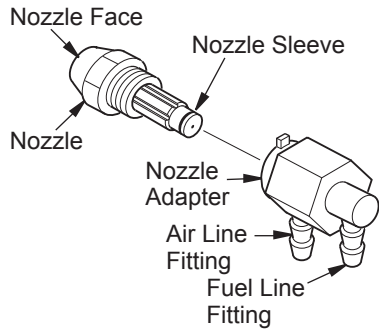
Figure 18 - Nozzle and Nozzle Adapter
