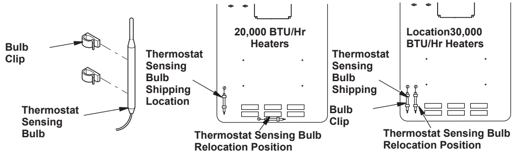
Figure 6 - Moving Thermostat Sensing Bulb Blue Flame Heaters Only
