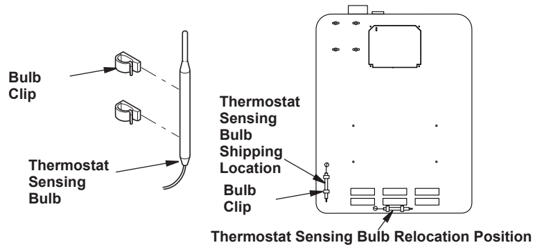
Figure 7 - Moving Thermostat Sensing Bulb Infrared Heaters Only
